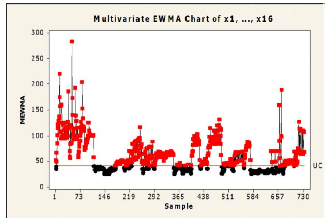
Fig. (2) MEWMA chart of x_1, \dots, x_{16} with ARL = 200, r = 0.3
